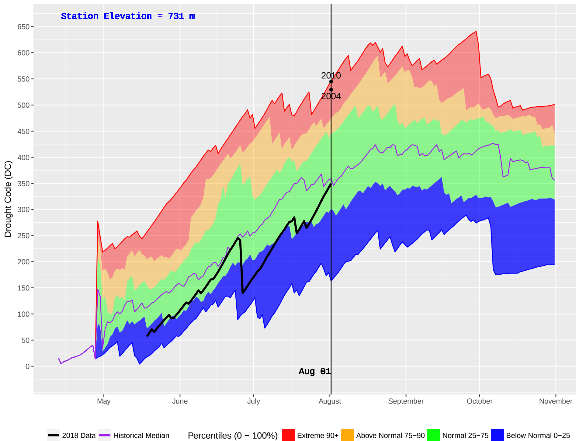
FIRESIDE (440) : Historical (1996–2016) and Current (2018) Daily Drought Code (DC)
