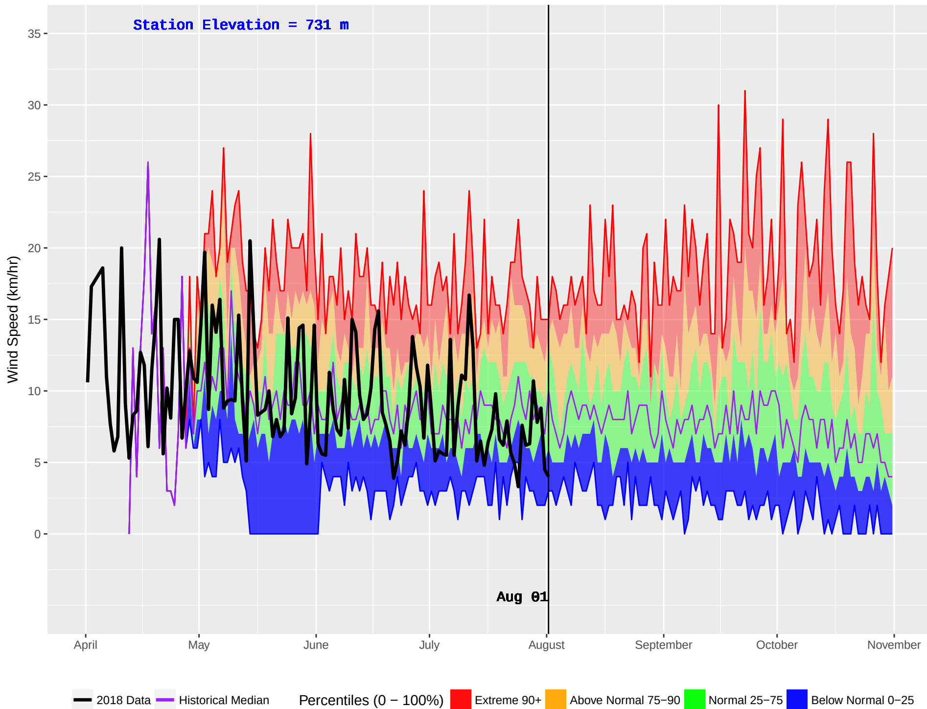
FIRESIDE (440) : Historical (1996–2016) and Current (2018) Daily Wind Speed
