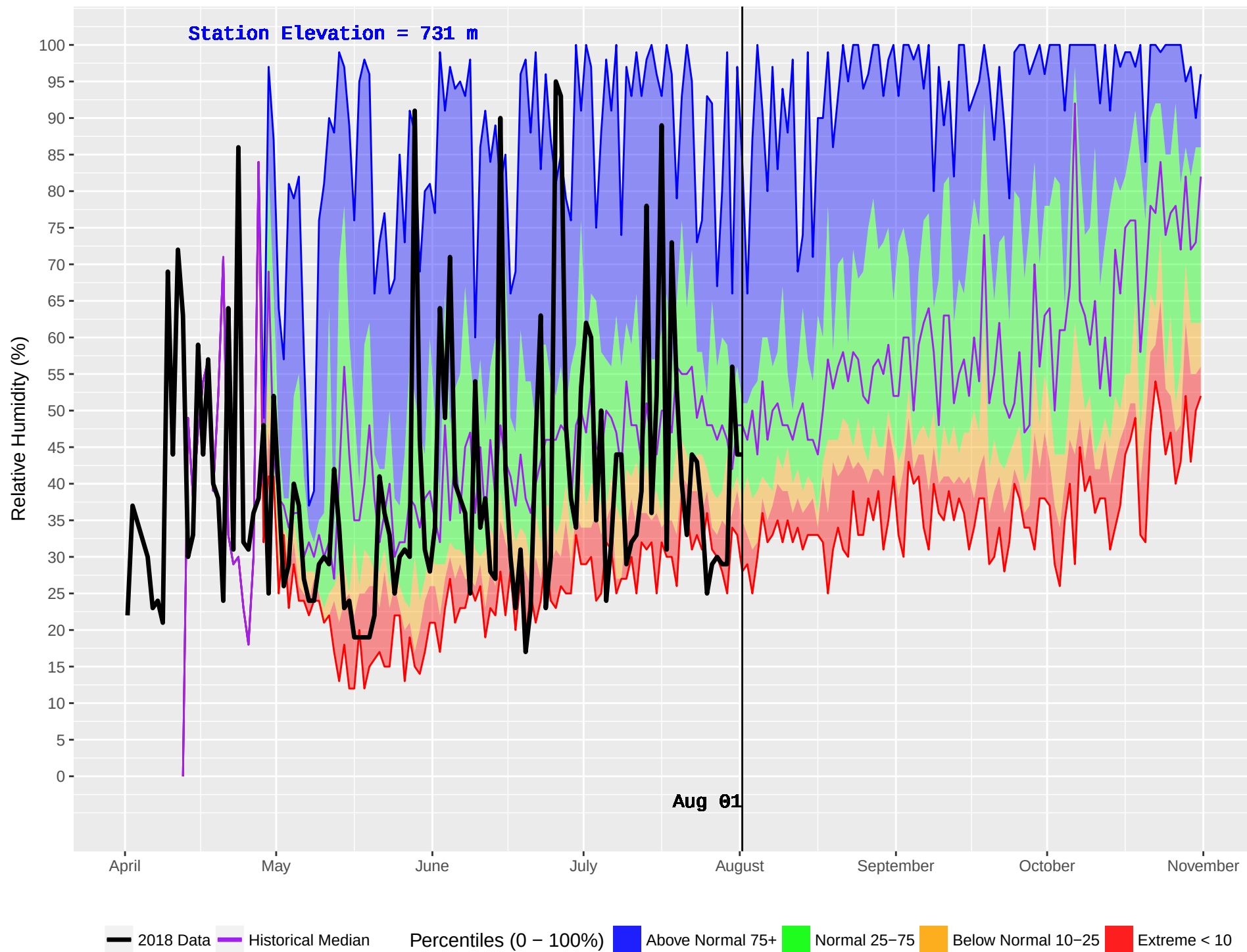
FIRESIDE (440) : Historical (1996–2016) and Current (2018) Daily Relative Humidity
