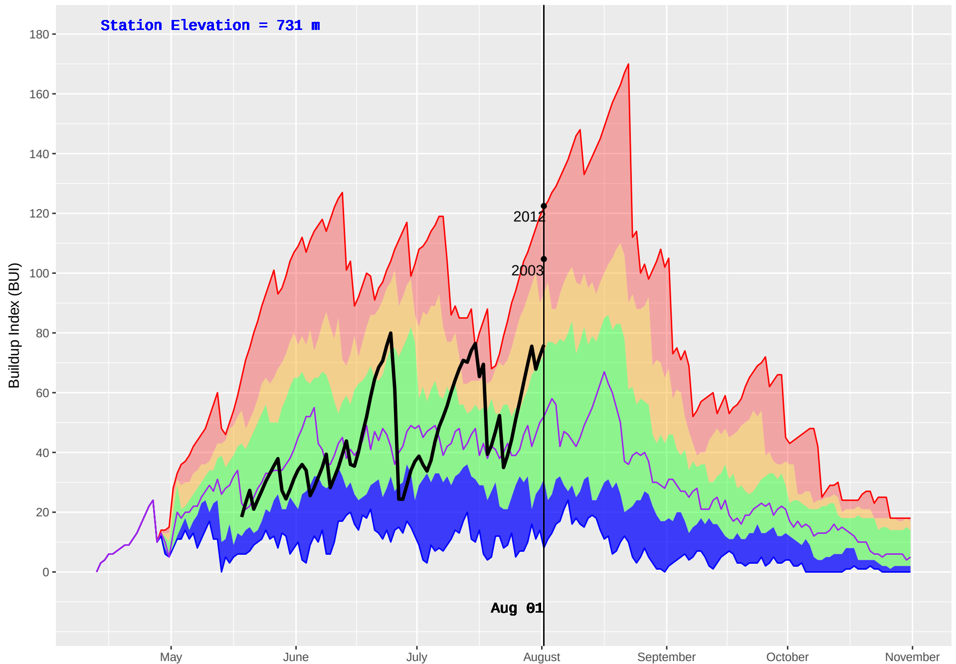
FIRESIDE (440) : Historical (1996–2016) and Current (2018) Daily Buildup Index (BUI)
