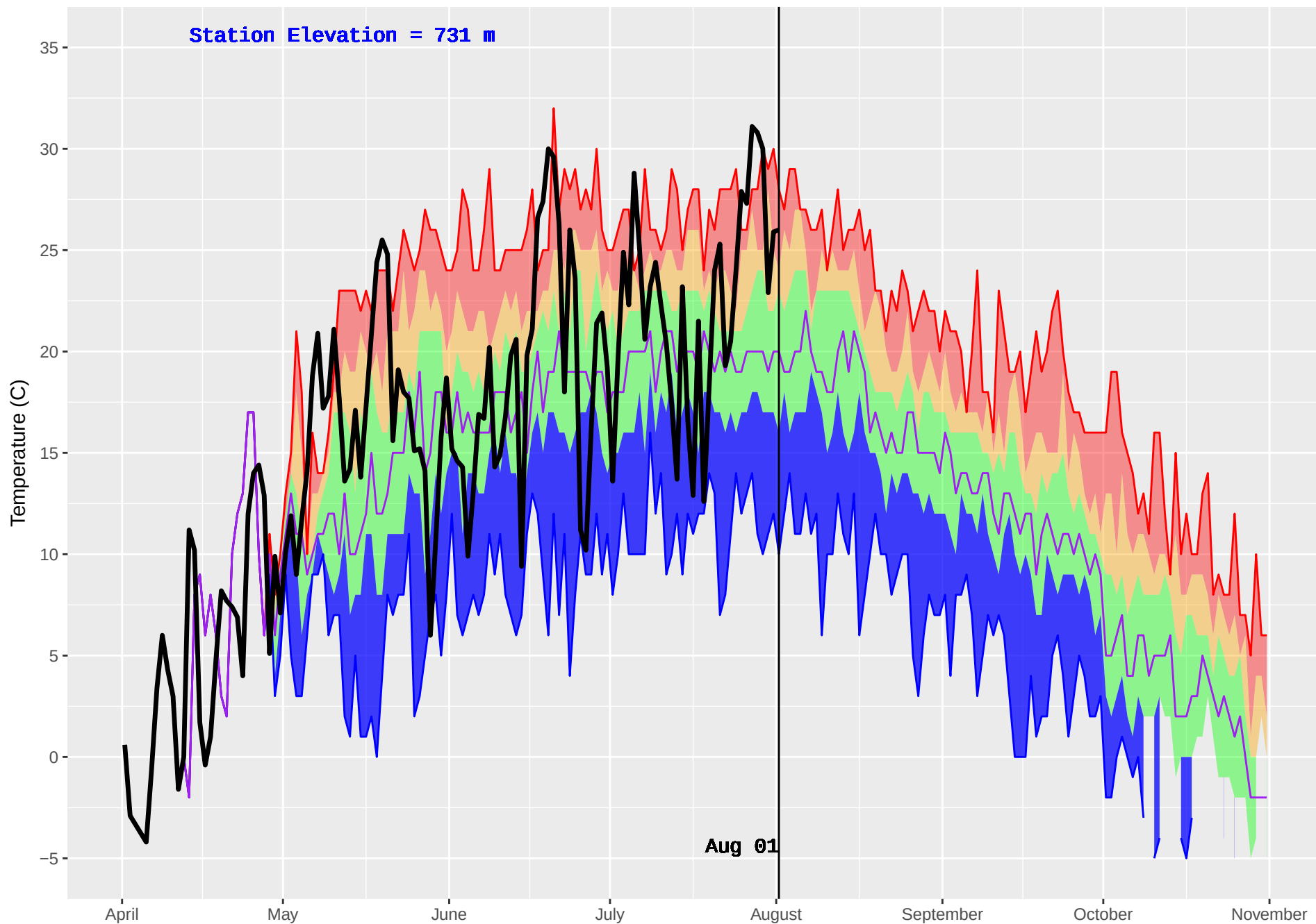
FIRESIDE (440) : Historical (1996–2016) and Current (2018) Daily Temperature
