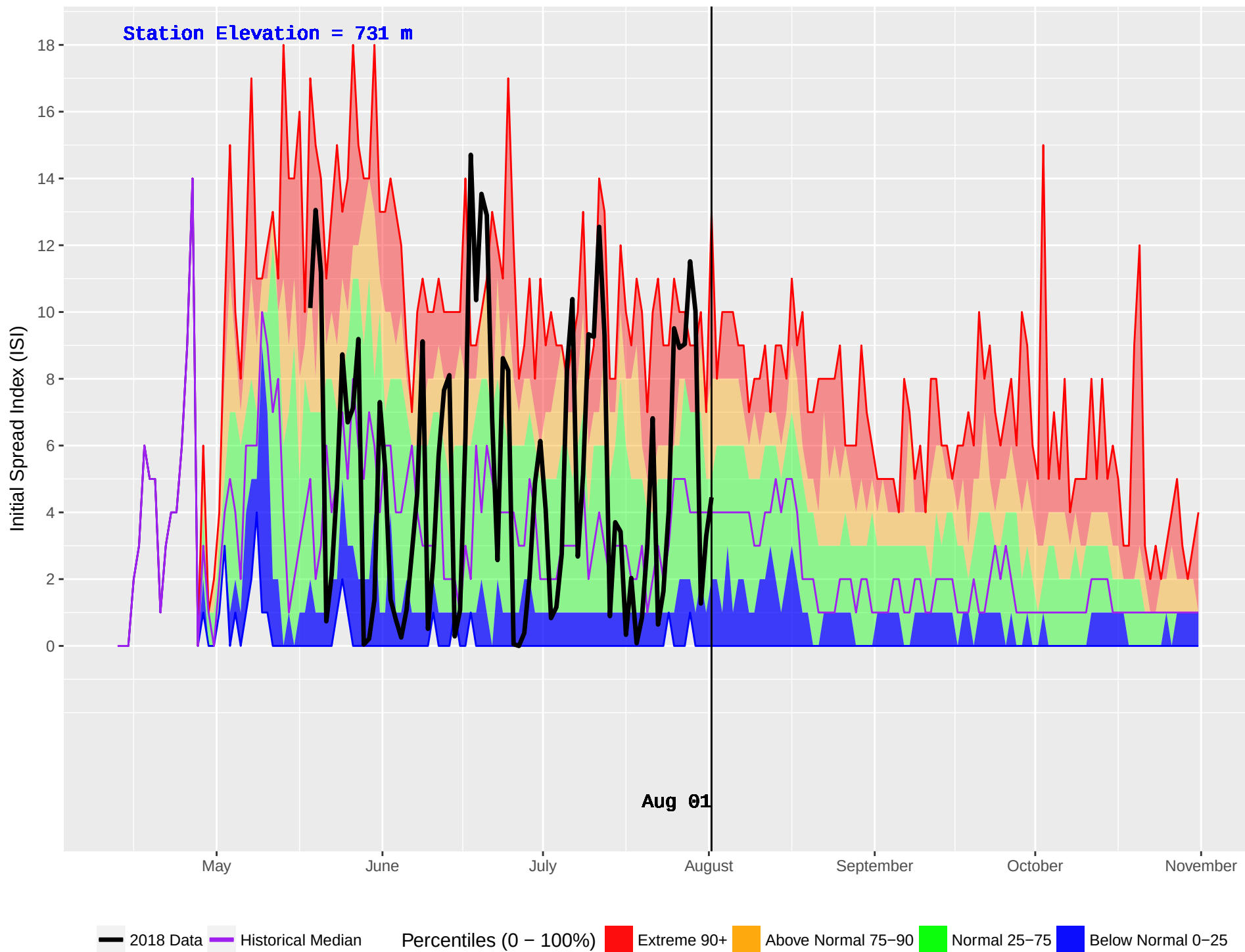
FIRESIDE (440) : Historical (1996–2016) and Current (2018) Daily Initial Spread Index (ISI)
