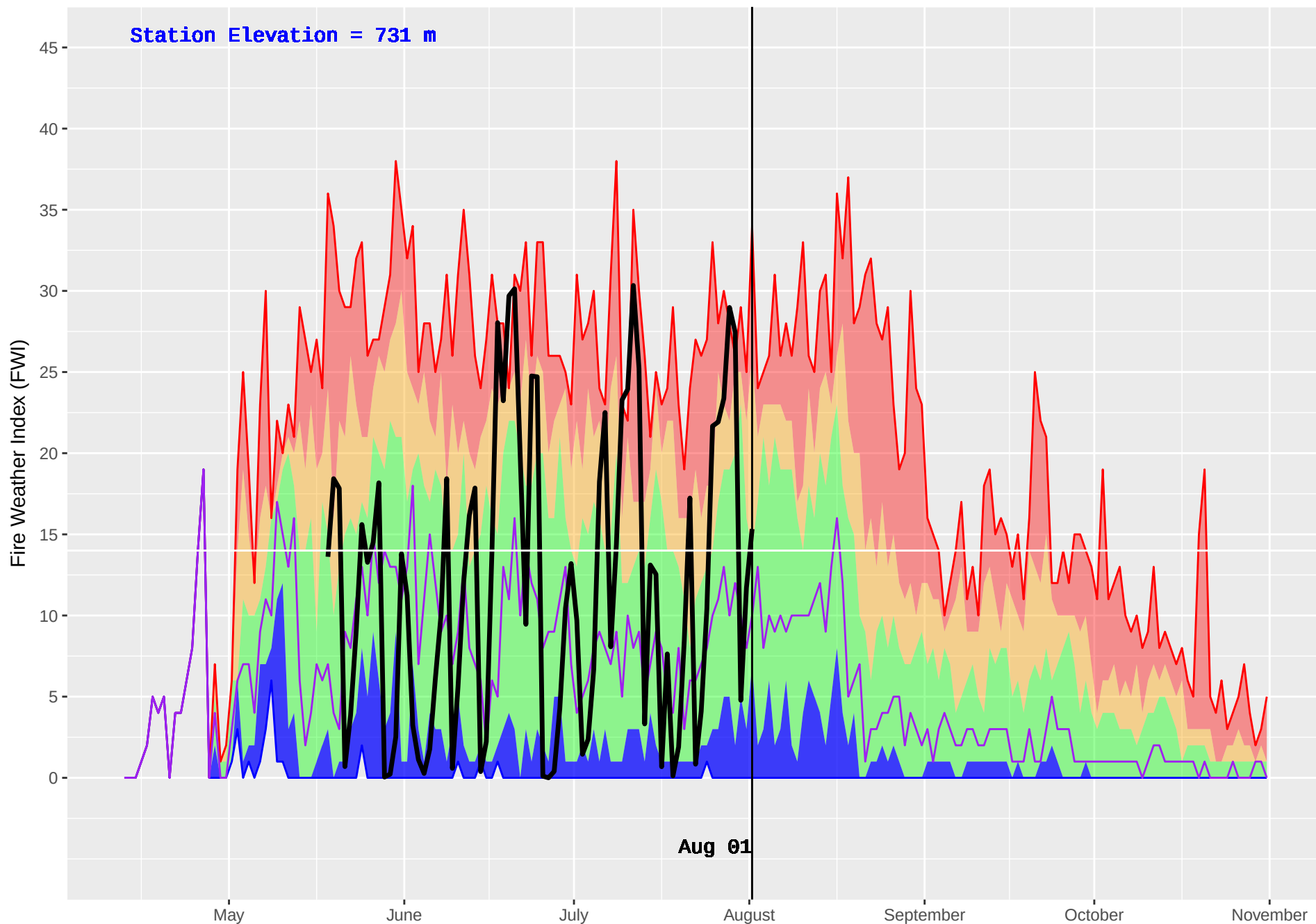
FIRESIDE (440) : Historical (1996–2016) and Current (2018) Daily Fire Weather Index (FWI)
